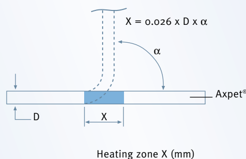
Fig. 8: Adjustment of heating zone
