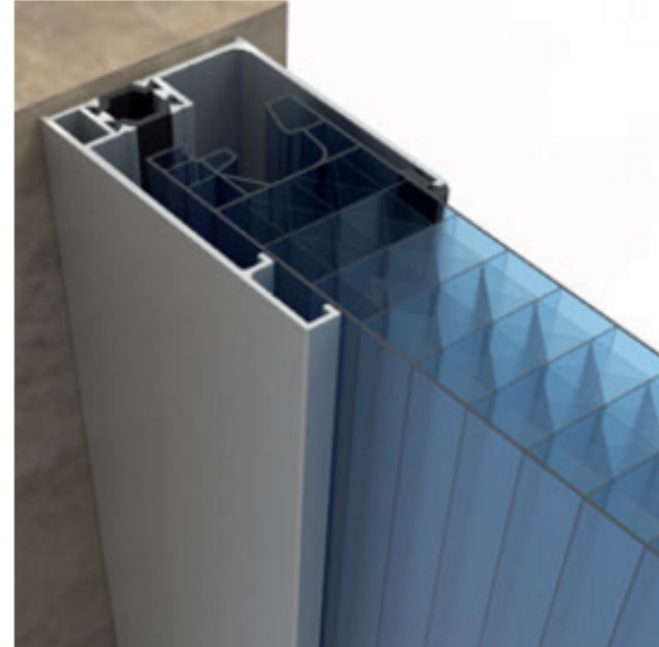
Detail side profile TT in AL
