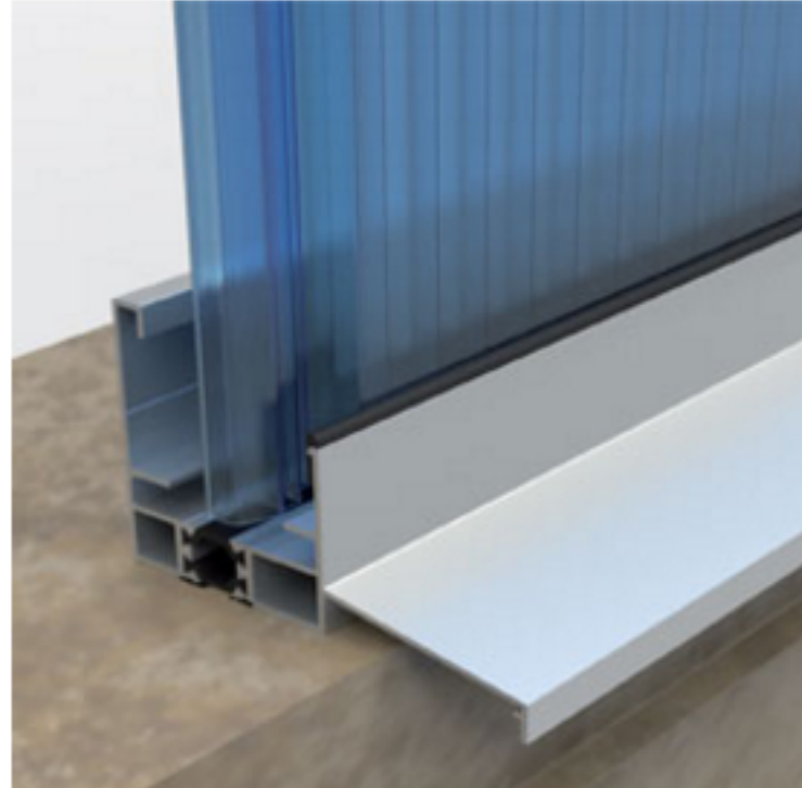
Detail base profile TT with eave in AL
