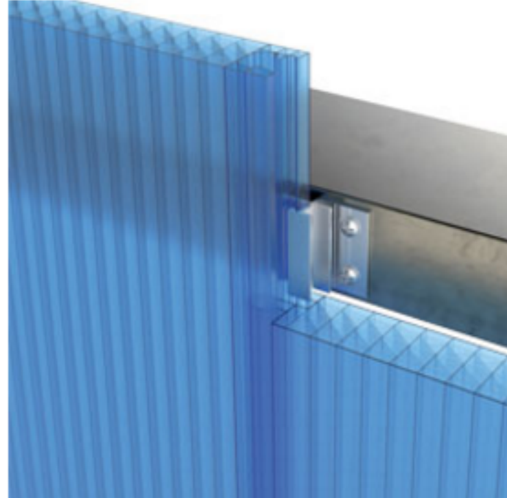
Anchorage to existing structures by inserting aluminum bracket
